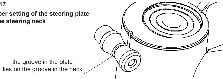
fig. 18 example of the correct positioning of the steering plates against each other
